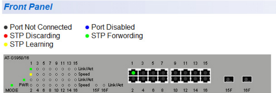
Figure 4. AT-GS950/16 Front Panel Page
